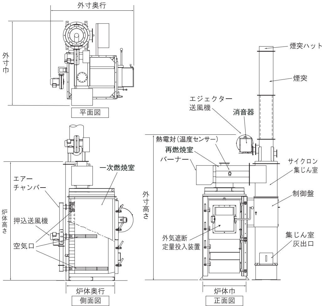
図面はAGZR-900M
